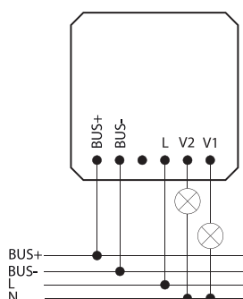
IBWL3-02B-SL
