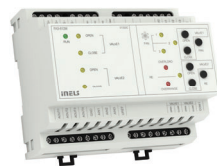
FA3-612M Controlador de fan coil
